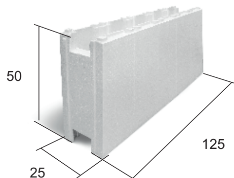
TrendStone L Standardstein Art-Nr. 18500/18505-SP
