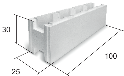
Easystone Standardstein Art-Nr. 18490-40-SP
